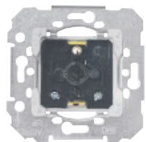
2 pole with socket outlet earth pin 18572 (French/Belgian standard) with increased touch protection Screwed terminals 16 A 250 V~
