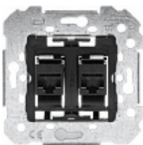
Adapter with 2 RJ45 connectors Cat. 6 Tool-less connection
