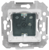
Schuko® socket outlet 18524 with increased touch protection Screwed terminals 16 A 250 V~
