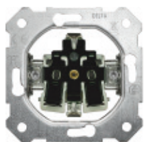
Schuko® socket outlet 5UB1101-5B with screw-less terminals with claws Schuko® socket outlet 5UB1101-5KK with screw-less terminals without claws
