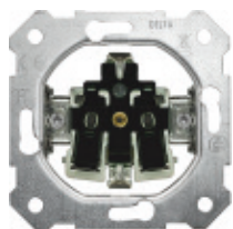
Schuko® socket outlet 5UB1101-5B with screw-less terminals with claws
